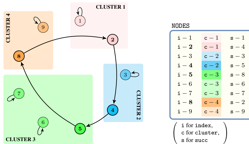
Figure 5.165: Four clusters and a covering with one circuit corresponding to the first example of the Example slot
