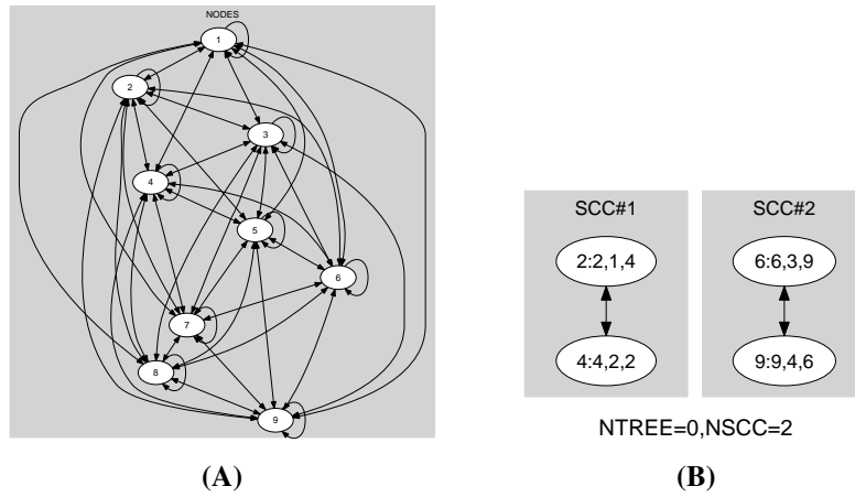
Figure 5.167: Initial and final graph of the circuit_cluster constraint
