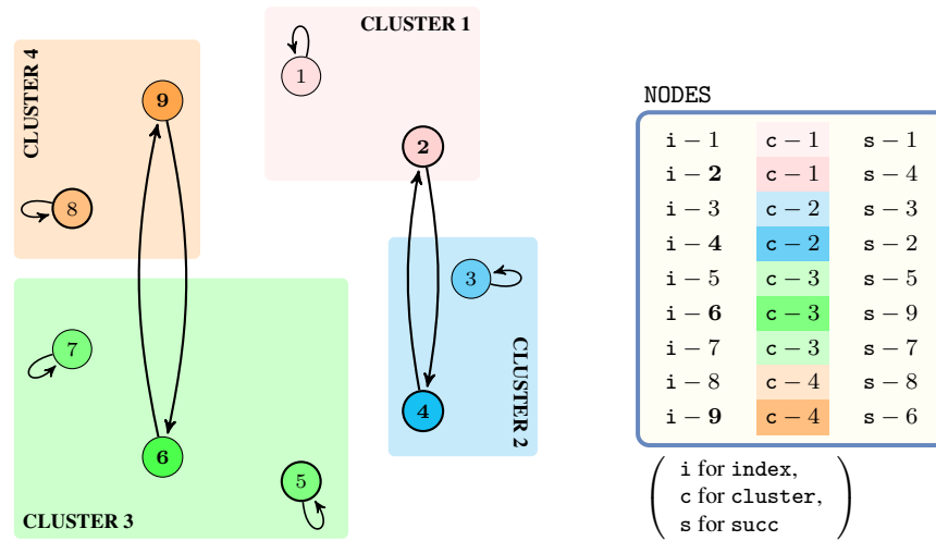
Figure 5.166: The same clusters as in the first example of the Example slot and a covering with two circuits corresponding to the second example of the Example slot
