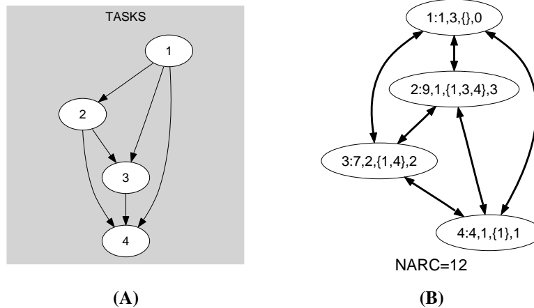
Figure 5.274: Initial and final graph of the disj constraint
