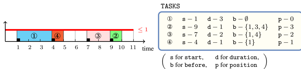
Figure 5.273: Tasks corresponding to the Example slot
