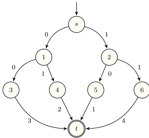
Figure 5.191: Automaton associated with the preference table of the cond_lex_less constraint given in the Example slot
