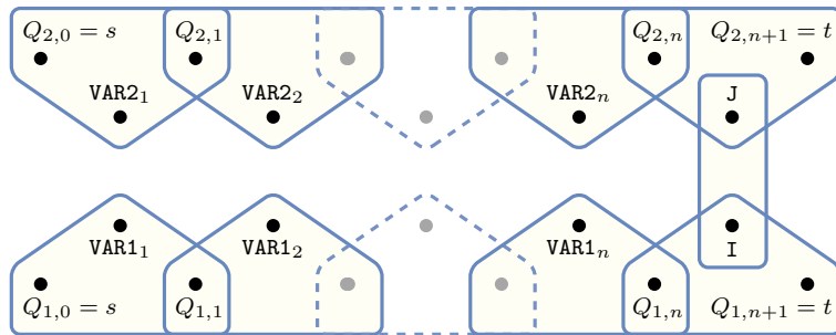
Figure 5.192: Hypergraph of the reformulation corresponding to the cond_lex_less constraint: it uses two occurrences of the automaton of Figure 5.191 and the constraint I < J
